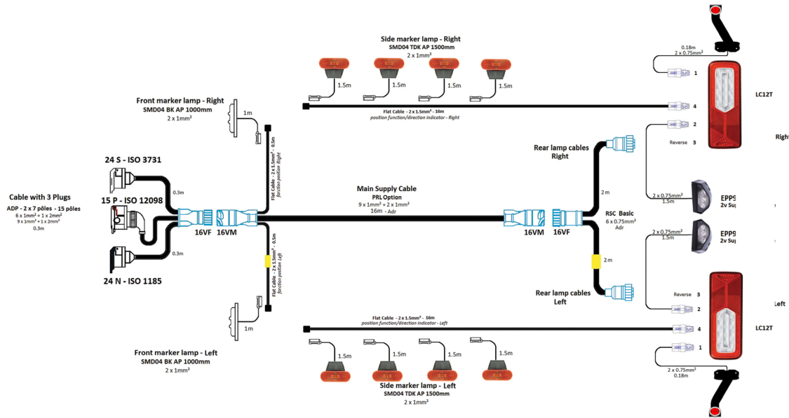
GRANDE REMORQUE 8 FEUX DE POSITION 100% LED Ref. VIGN A13888
